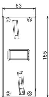
Gettoniera frontalino alto (per M10 e M20) High front plate for Coin Selector (for M10 and M20)
